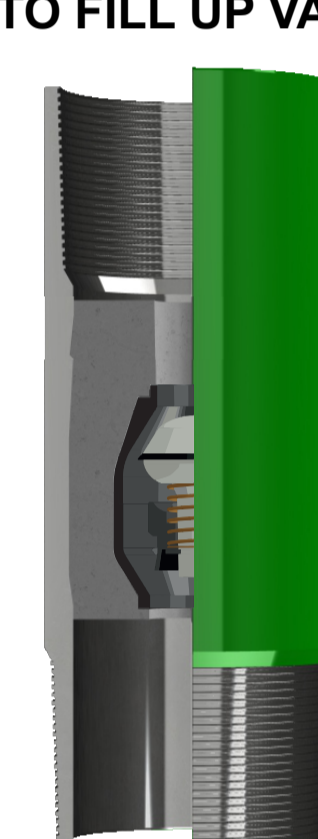
FLOAT COLLAR AUTO FILL UP VALVE
