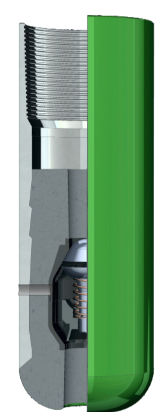
FLOAT SHOE SIDE JET
