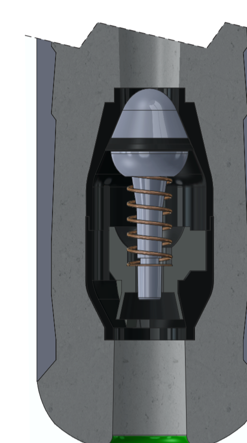
PLUNGER VALVE
