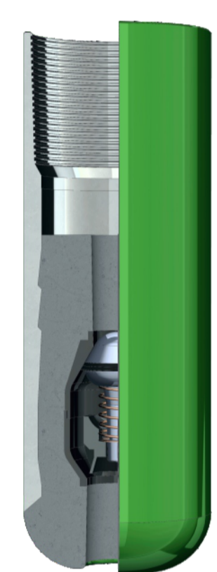
FLOAT SHOE PLUNGER VALVE
