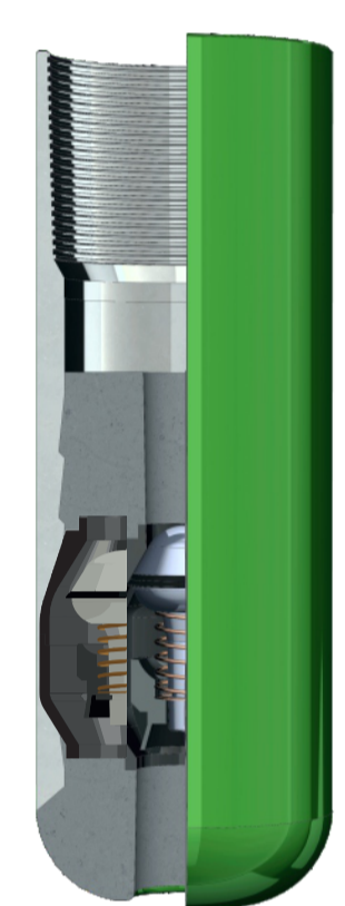
FLOAT SHOE AUTO FILL UP VALVE
