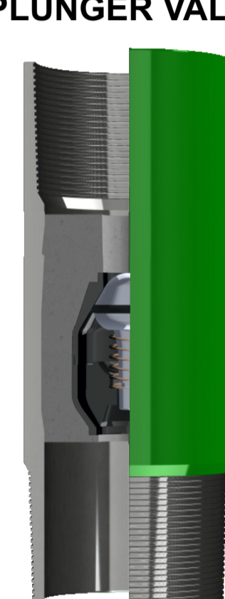
FLOAT COLLAR PLUNGER VALVE
